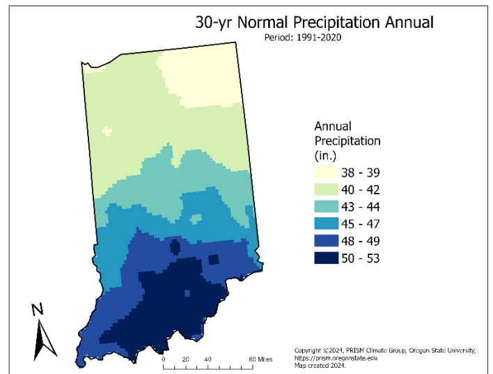
Figure 3. Normal mean precipitation (in.) from 1991–2020 in Indiana.
