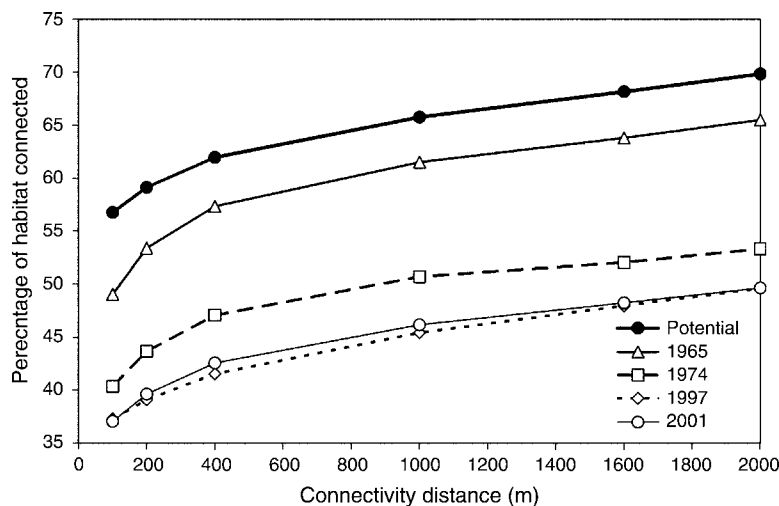
FIG. 6. Percentage of the total habitat (including marginally, moderately, and highly suitable) connected within the eastern boundary area vs. distance between patches (connectivity) of panda habitat for each of the dates of imagery analyzed and for the potential habitat modeled.
