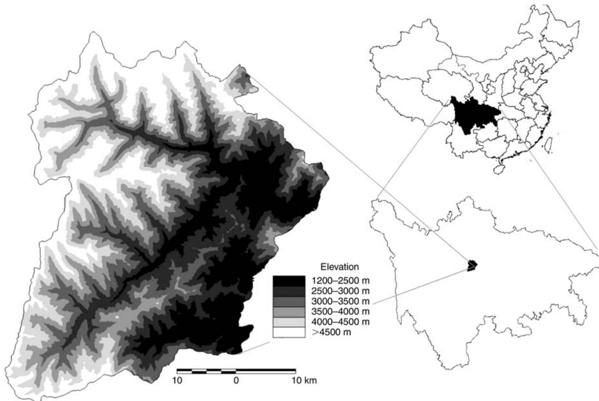
FIG. 1. Location and topography of the Wolong Nature Reserve in Sichuan Province, China.
